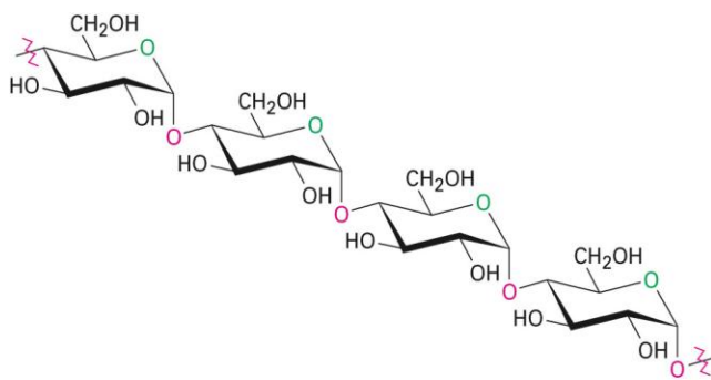
Amylose, a 1→4-O-( \alpha -D-glucopyranoside) polymer
