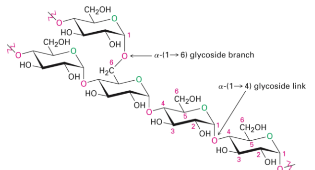
Amylopectin: \alpha -(1→4) links with \alpha -(1→6) branches
